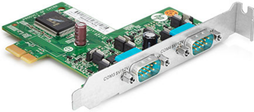
HP RS232-card for HP rp5800 #QP906AA
